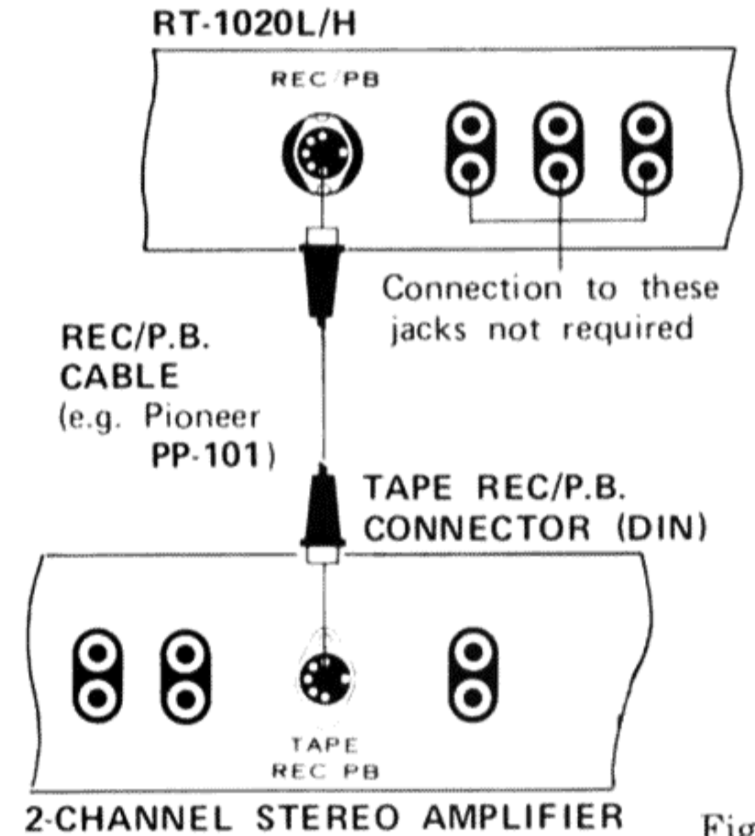
JACKS OF 2-CHANNEL STEREO AMPLIFIER Fig. 6
