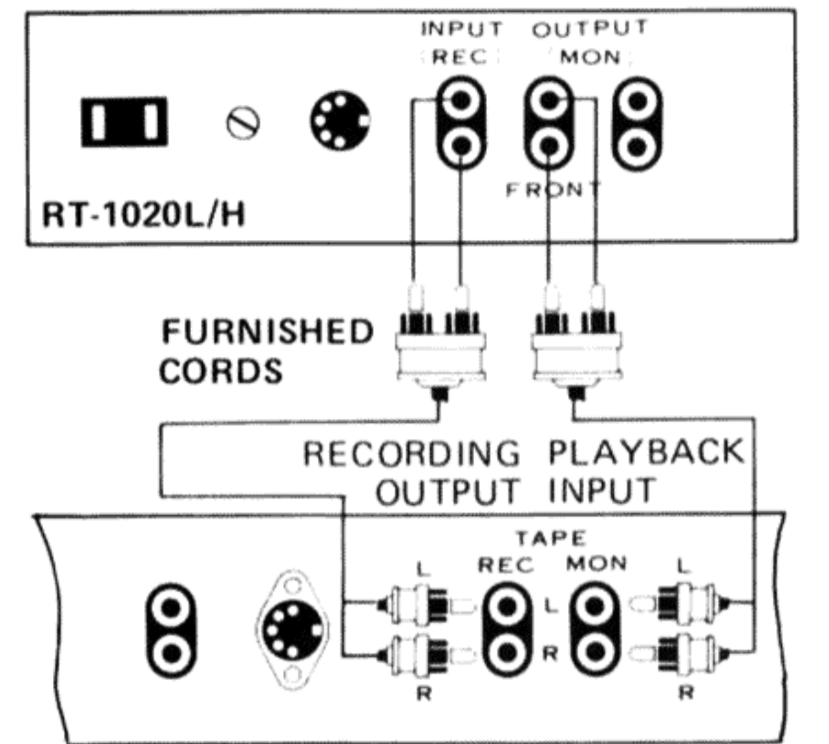
JACKS OF 2-CHANNEL STEREO AMPLIFIER Fig. 6
