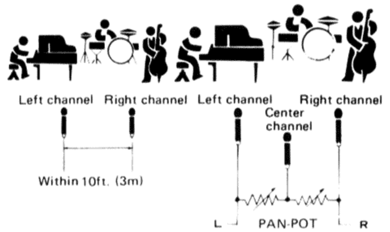
Vacant center avoided by using center microphone Fig. 3-B
